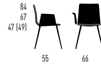
CHAIR WITH ARMRESTS WITH UPHOLSTERED ARMRESTS
