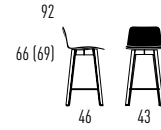
COUNTER STOOL HIGH (HIGH BACKREST)
