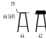
COUNTER STOOL LOW (LOW BACKREST)
