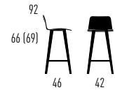
COUNTER STOOL HIGH (HIGH BACKREST)
