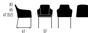
CHAIR WITH ARMRESTS WITH UPHOLSTERED ARMRESTS
